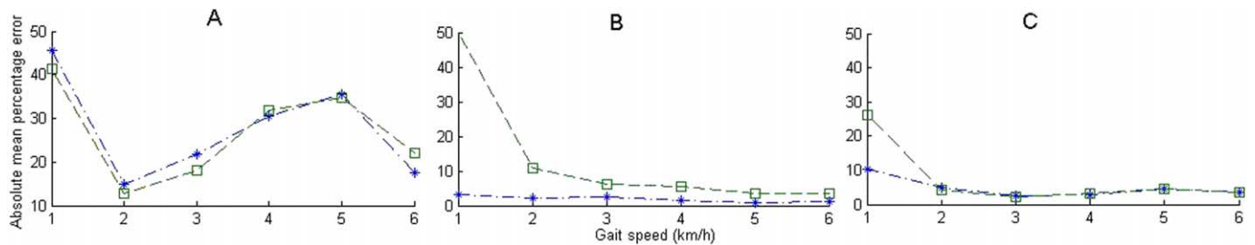
Figure 3: Results for the superimposed autocorrelation in comparison to autocorrelation at different time windows and at a wide range of gait speeds. Superimposed autocorrelation = □ and regular autocorrelation = *. A = 2 seconds TW, B = 4 seconds TW and C = 8 seconds TW. Data is presented as the mean absolute percentage error against camera observation.
