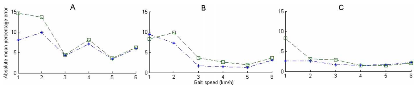
Figure 4: Results for the superimposed PSD in comparison to PSD at different time windows and at different gait speeds. Superimposed PSD = □ and regular PSD = *. Respectively A = 2 seconds TW, B = 4 seconds TW and C = 8 seconds TW. Data is presented as the mean absolute percentage error against camera observation.
